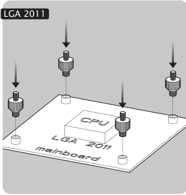
Fasten LGA 2011 screws tightly onto MB.
