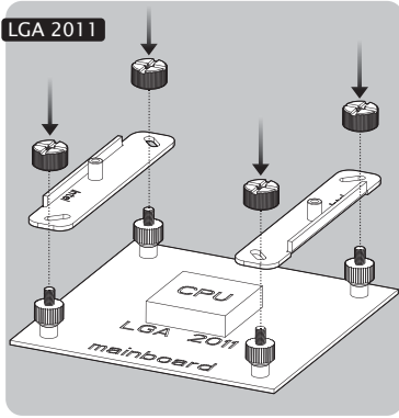
Aim the holes of Intel mounting-clip to the LGA 2011 screws, and slip over the clips to the screw. Then, fasten the metal nuts onto LGA 2011 screws.
