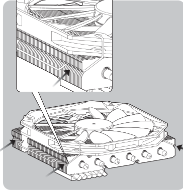
Utilize fan clips to buckle fan securely onto heat-sink
