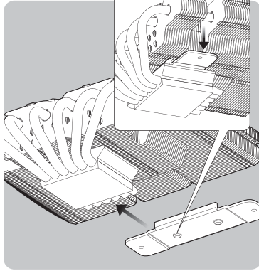
Cross the crossbar thru above the Heat-sink base, and aim the raise points of crossbar to holes of Heat-sink base.
