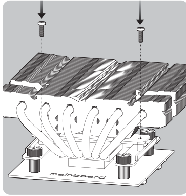
Aim the holes of crossbar to the pillar holes of mounting-clip, then use screw driver ⊕ and M3 screws to fasten cross bar and mounting-clips
