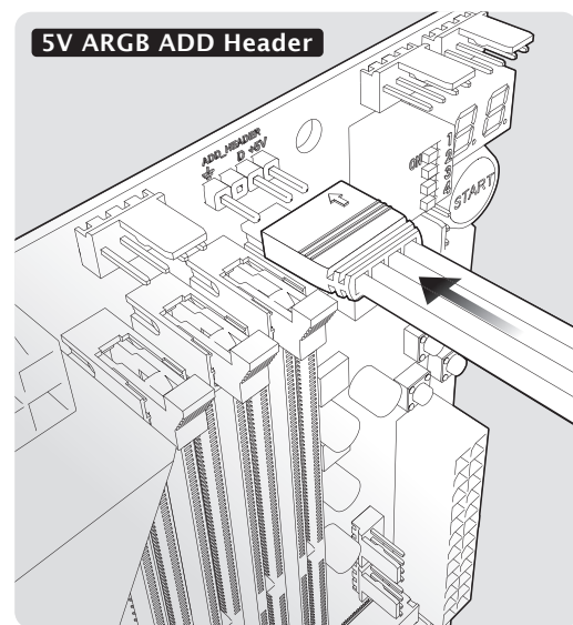
2 in 1 cable header
