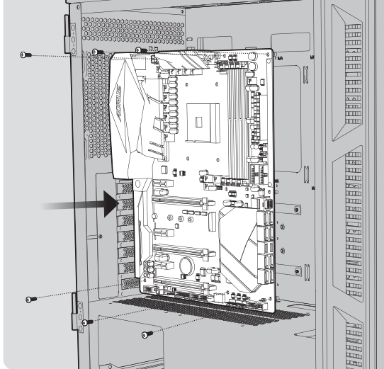
MOTHERBOARD
